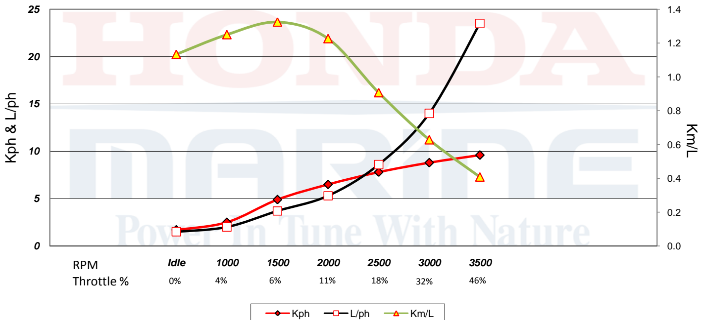
Bella Casa House Boat & BF135A4LD Average Speed & Fuel Consumption
